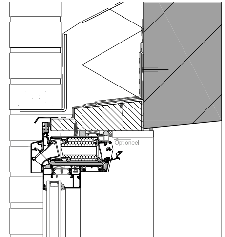
Detail Invisivent NL AK Basic [verborgen waterafvoer]
