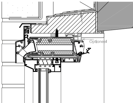
Detail Invisivent NL AK High [verborgen waterafvoer]
