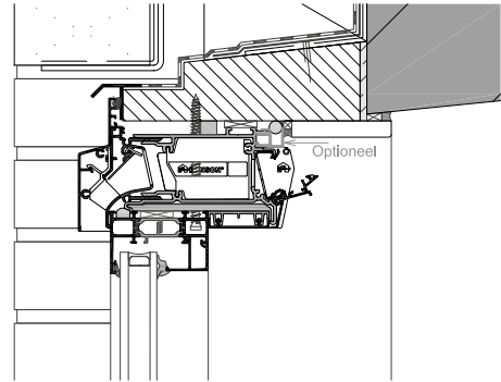
Detail Invisivent NL [zichtbare waterafvoer]
